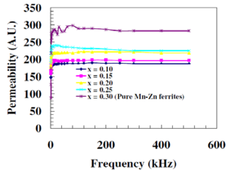
Fig. 3. Permeability versus frequency curves of \text{Mn}_x\text{Zn}_{0.4}\text{Ca}_{0.6-2x}\text{Fe}_{2+x}\text{O}_4 where, x = 0.10, 0.15, 0.20, 0.25 and 0.30 .
