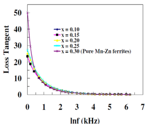
Fig. 5. Loss tangent of Mn_xZn_{0.4}Ca_{0.6-2x}Fe_{2+x}O_4 where x = 0.10, 0.15, 0.20, 0.25 and 0.30 as a function of frequency.
