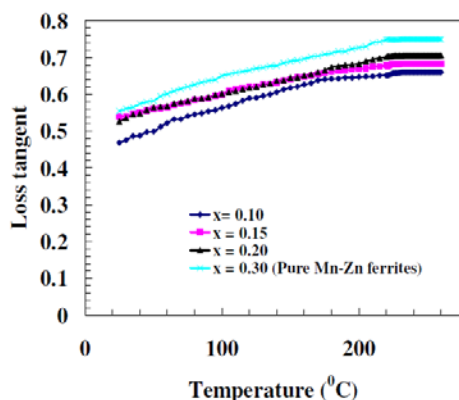
Fig. 4. Loss tangent of Mn_xZn_{0.4}Ca_{0.6-2x}Fe_{2+x}O_4 where x = 0.10, 0.15, 0.20, and 0.30 as a function of temperature.
