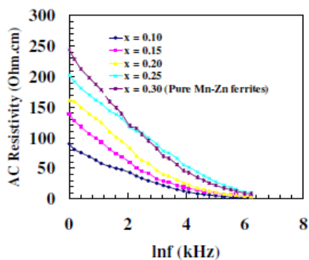
Fig. 9. AC resistivity of \text{Mn}_x\text{Zn}_{0.4}\text{Ca}_{0.6-2x}\text{Fe}_{2+x}\text{O}_4 where x = 0.10, 0.15, 0.20, 0.25 and 0.30 as a function of frequency.
