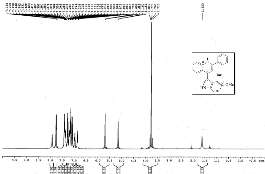
1 H-NMR of 3ae
