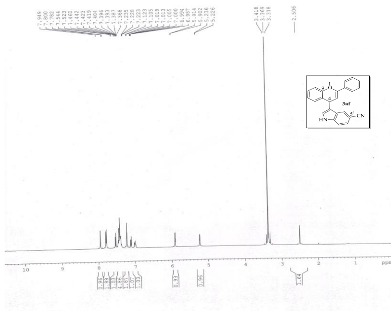
^1\text{H-NMR} of 3af
