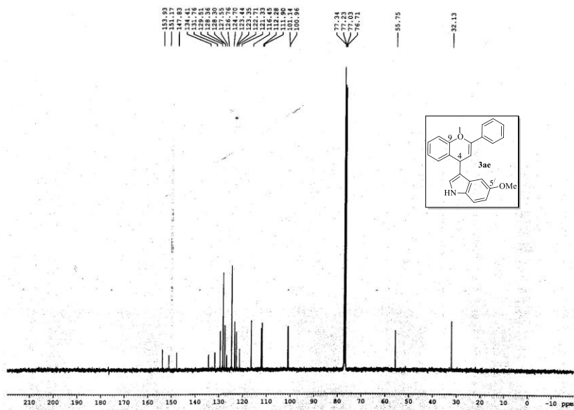
13 C-NMR of 3ae
