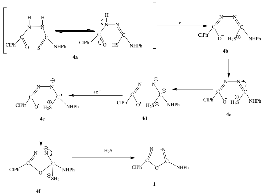
Scheme 2. Mechanistic proposal
