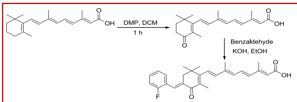
Scheme 1: Synthesis of 2-florobenzaldehyde retinoic acid chalcone
