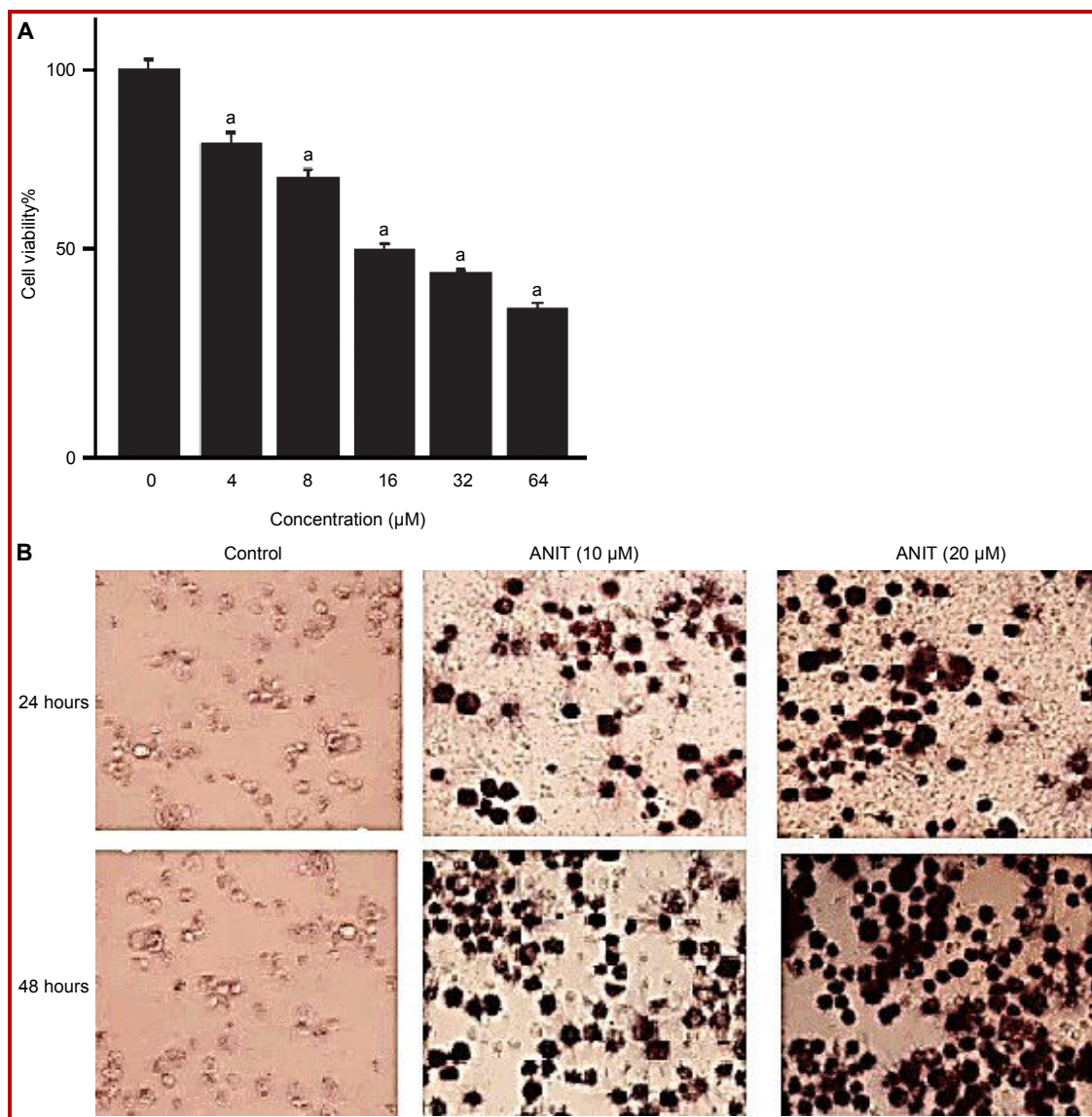
Figure 1: Effects of ANIT on cell viability (A) and morphology (B) of U87MG cells. Cells were cultured with 0, 4, 8, 16, 32 and 64 \mu\text{M} of ANIT for 24 hours
